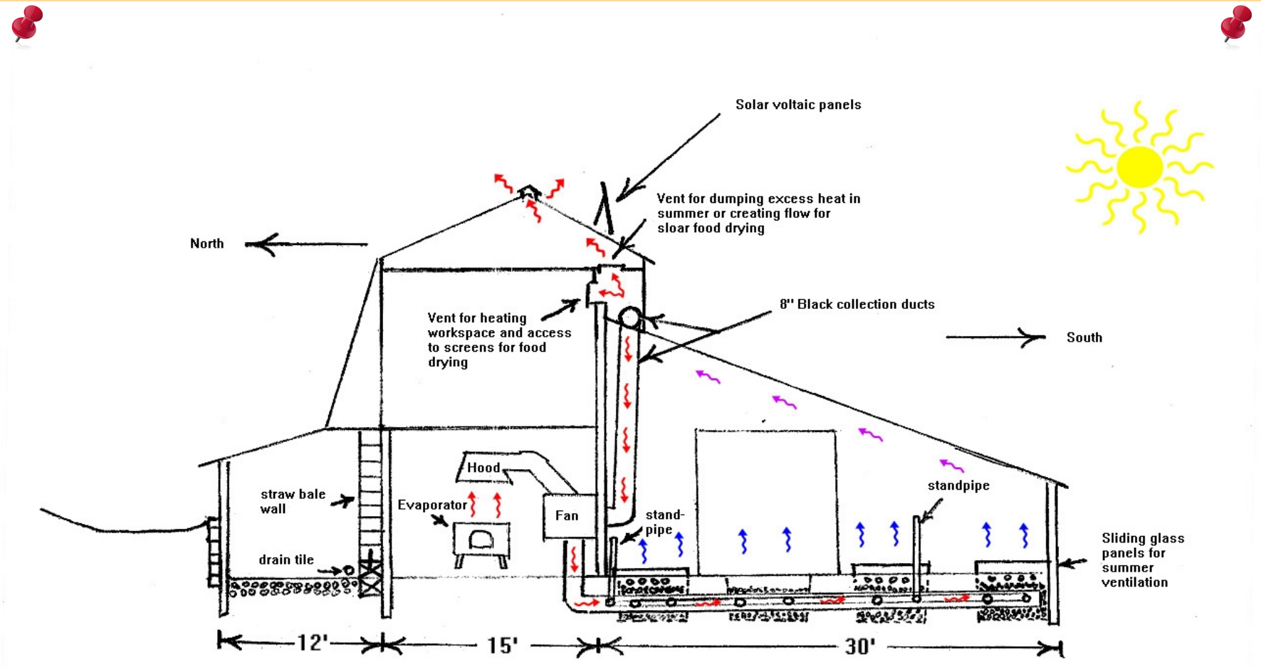
Diagram 1. End view showing air flow (squiggly arrows) from ridge through gravel and soil mix of growing beds.
