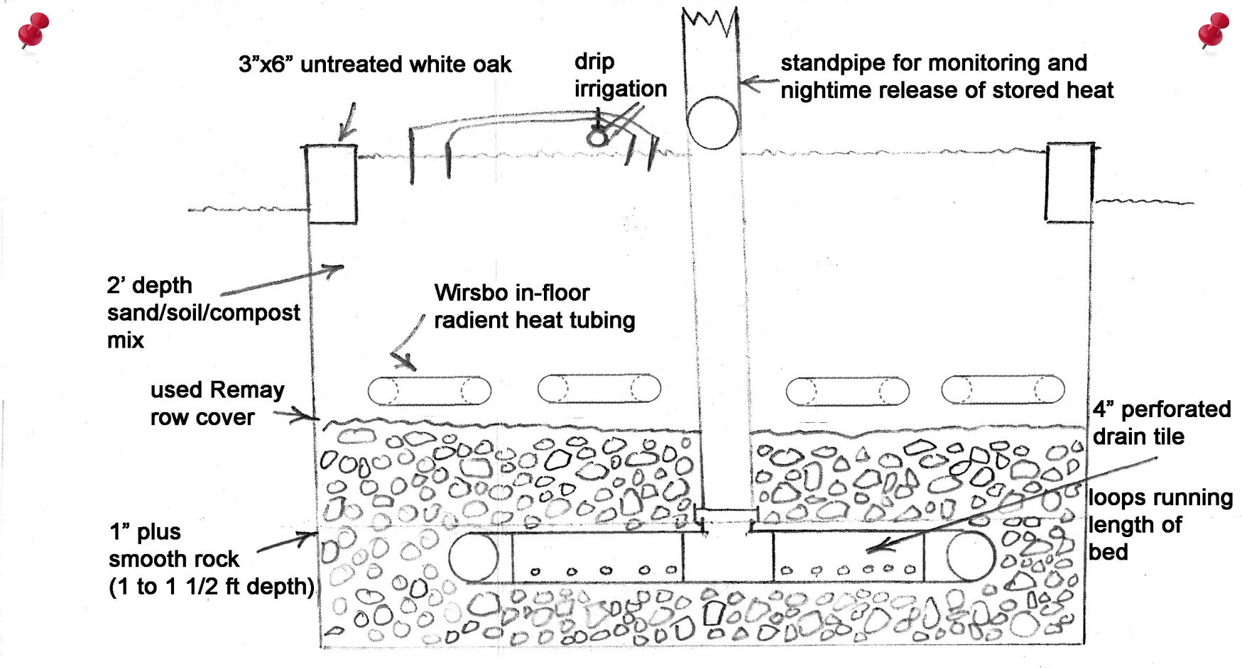
Diagram 2. Growing bed design and composition.
