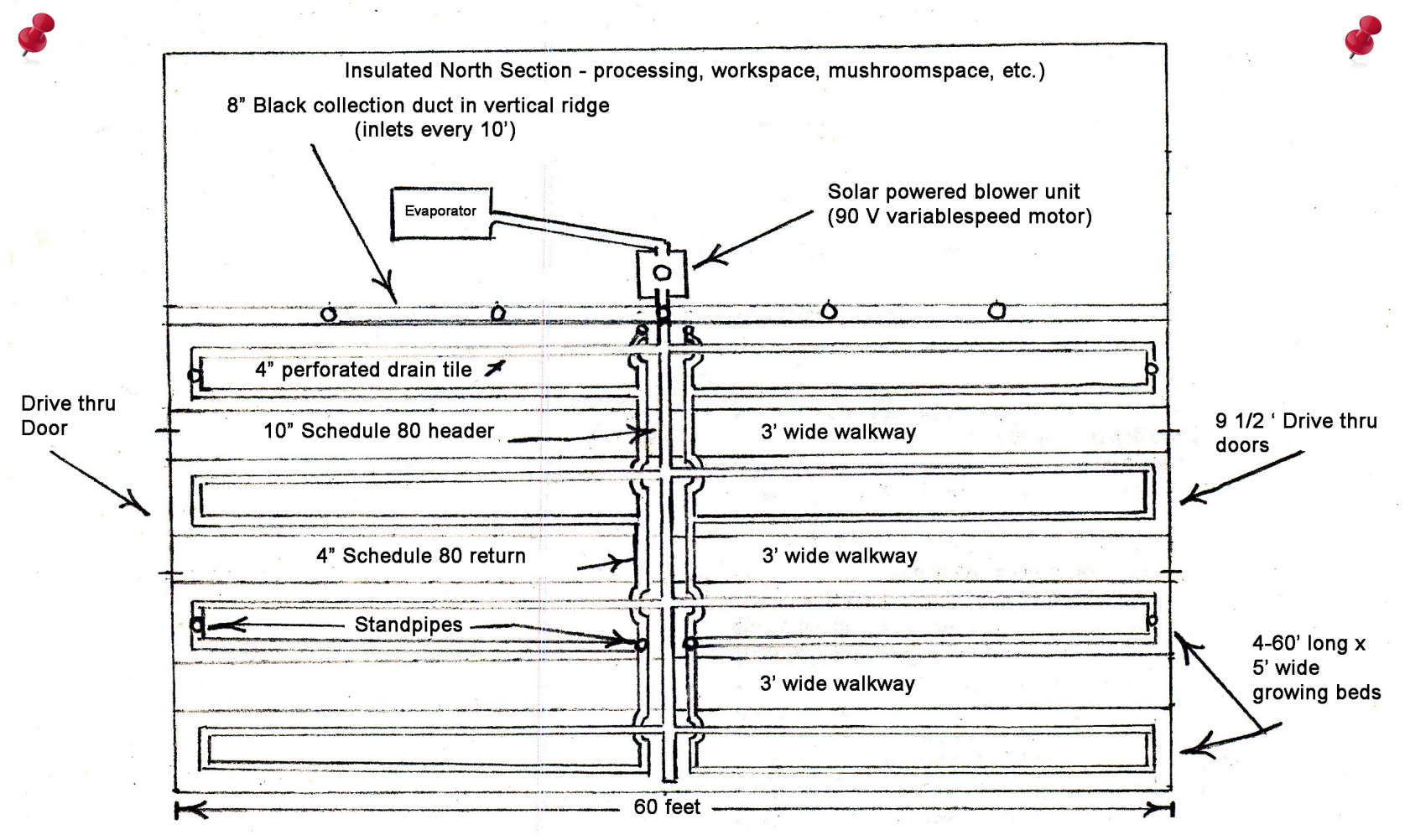
Diagram 3. Overhead view, layout of buried and above ground air collection system.
